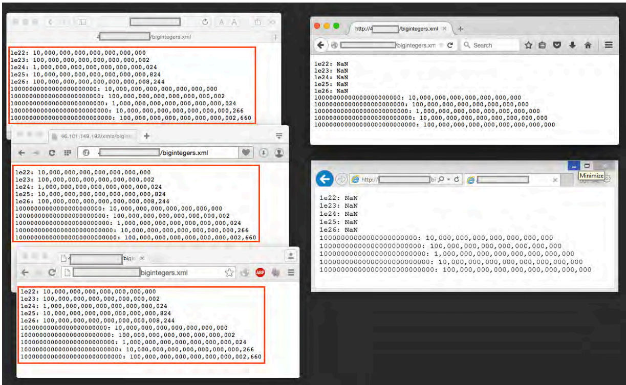
Figure 7: web browser showing incorrect values
