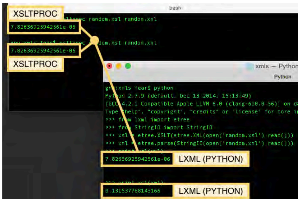
Figure 16: Random output using the same IV
