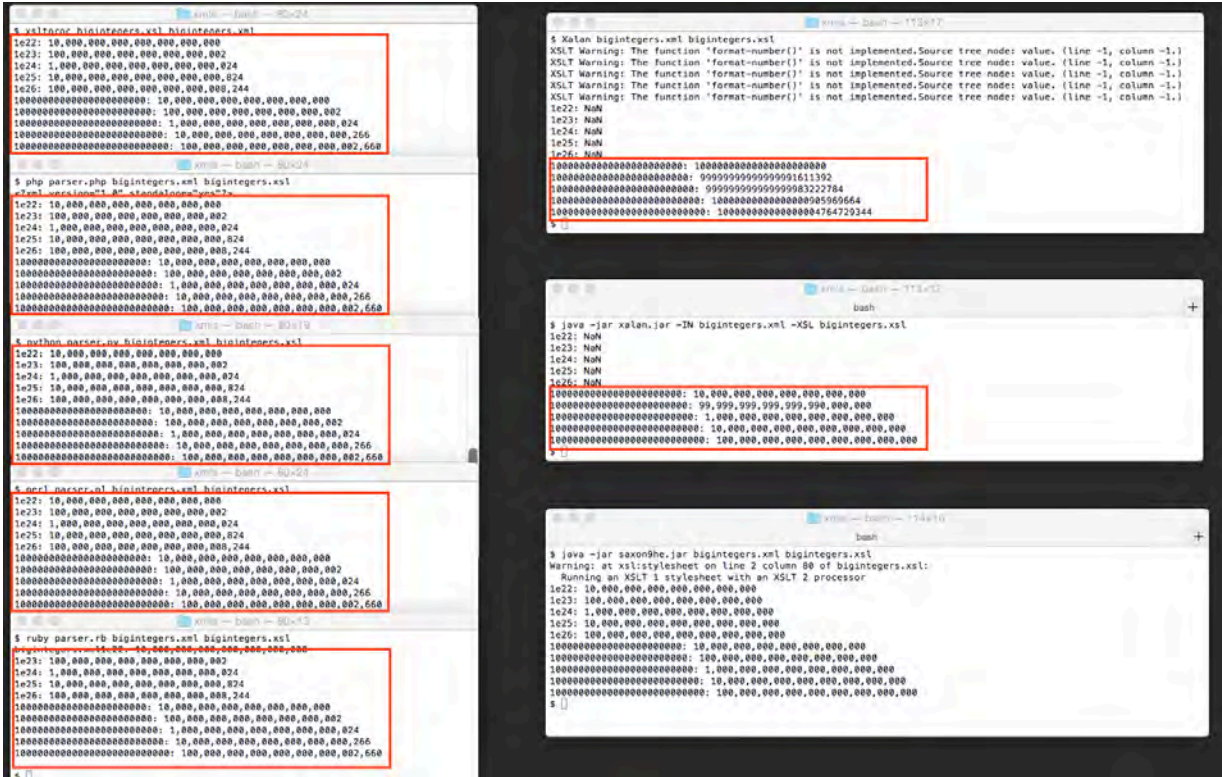
Figure 8: server side processors showing incorrect values
