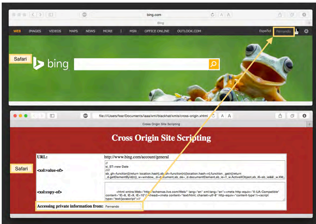
Figure 18: Reading Information from Bing
